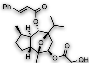
(-)-englerin A
