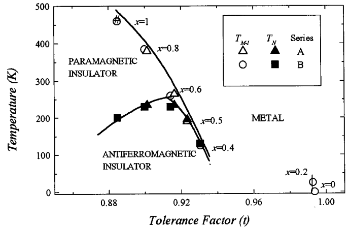
FIG. 11. Phase diagram of La 1– x Eu x NiO 3 obtained from crystallographic, magnetic, and electrical data.
