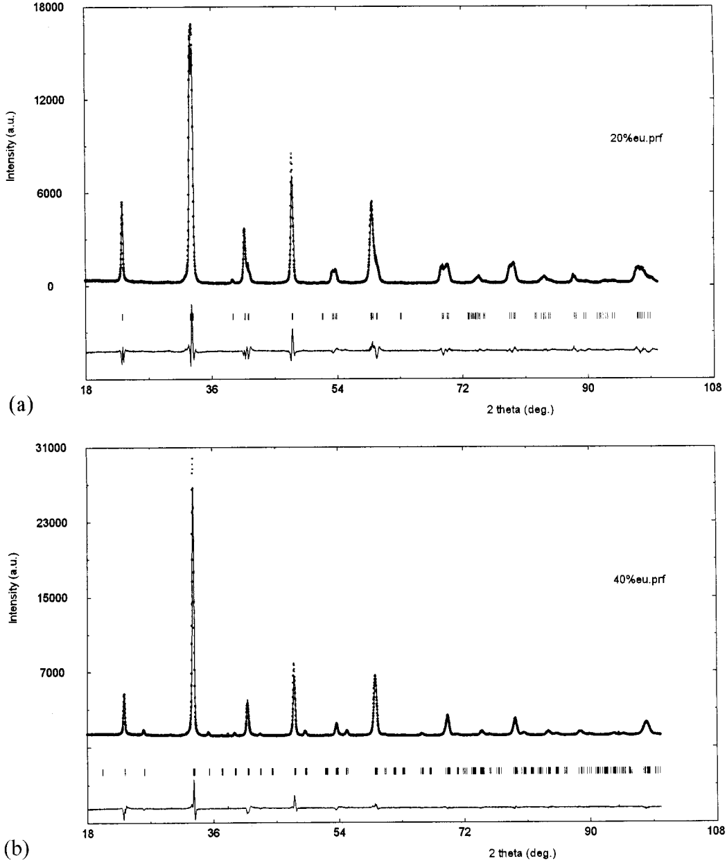
FIG. 2. Rietveld refined XRD patterns for (a) \text{La}_{0.8}\text{Eu}_{0.2}\text{NiO}_3 (space group R\bar{3}c ) and (b) \text{La}_{0.6}\text{Eu}_{0.4}\text{NiO}_3 (space group P6_{3}mm ).
