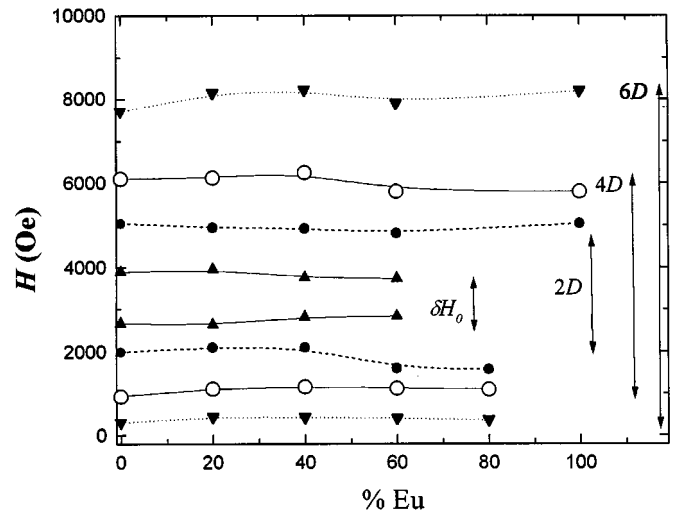
FIG. 10. Position of the resonance lines for the \text{La}_{1-x}\text{Eu}_x\text{NiO}_3 : \text{Gd}^{3+} series as a function of %Eu (or x ).
