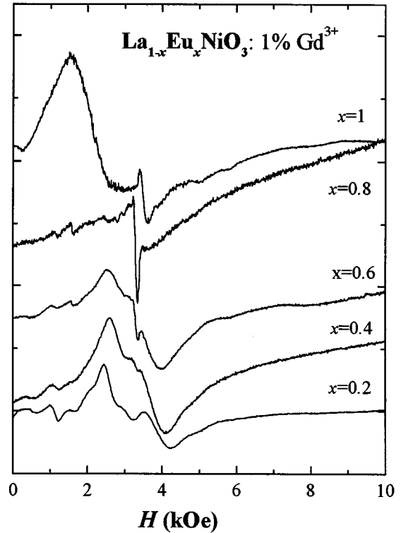
FIG. 8. ESR spectra of Gd 3+ in \text{La}_{1-x}\text{Eu}_x\text{NiO}_3 : Gd 3+ taken at liquid helium temperature. The x values are indicated in the plot.
