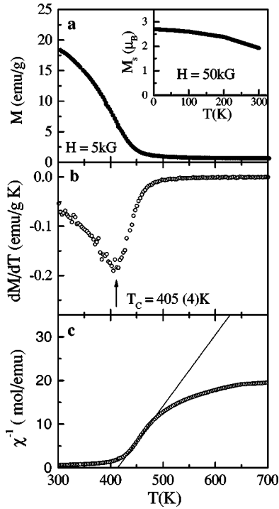
FIG. 3. Temperature dependence of (a) M ( H = 5 kG). The inset shows the saturated magnetization at low T . (b) dM/dT determining the Curie temperature ( T_C ). (c) Inverse of susceptibility. The straight line shows a fit with a Curie-Weiss law and the determination of the Curie-Weiss temperature ( \Theta = 416 K).
