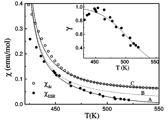
FIG. 8. ESR susceptibility \chi_{\text{ESR}} (solid circles) and \chi_{\text{dc}} data (open circles) as a function of temperature. The solid line A is the fit \chi_{\text{loc}} = \gamma(T)C_{\text{Fe}^{3+}} / (T - \Theta) , with \gamma(T) as shown in the inset. The dotted line B is the Curie-Weiss law for the \text{Fe}^{3+} ions and curve C is \chi_{\text{loc}} + \chi_{\text{itin}} (see text).
