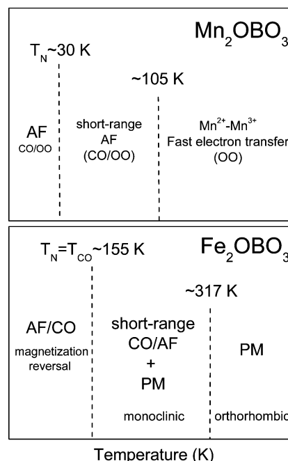
Figure 7. Schematic revised phase diagram proposed for Mn_2OBO_3 and Fe_2OBO_3 .
