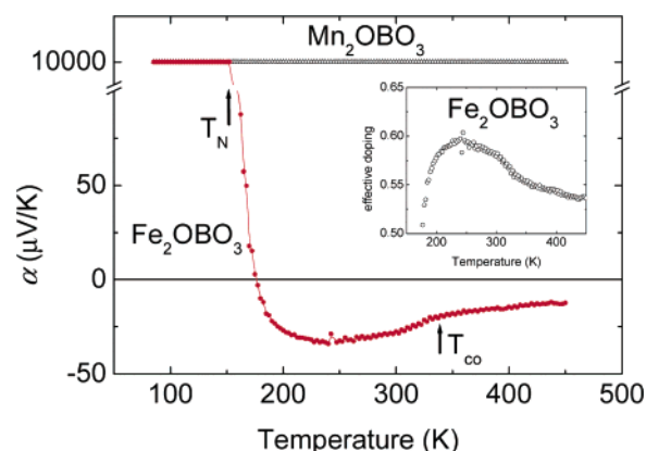
Figure 4. Thermoelectric power of Mn_2OBO_3 (open triangles) and Fe_2OBO_3 (closed circles). Inset: effective doping from thermopower in Fe_2OBO_3 .
