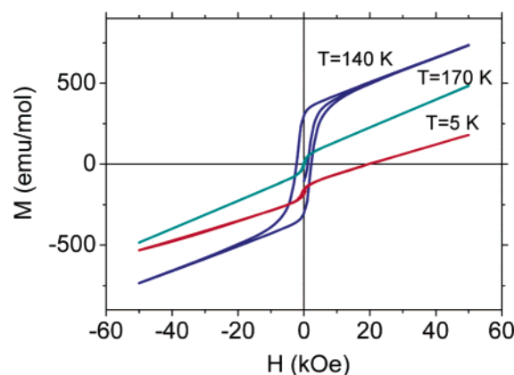
Figure 6. ZFC magnetization versus applied field H of \text{Fe}_2\text{OBO}_3 measured at three different temperatures, T = 5 , 140, and 170 K.
