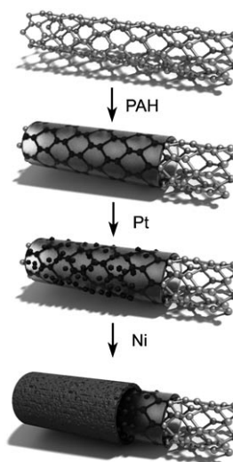
Figure 1. Illustration of the synthetic process comprising the polymer (PAH) wrapping of CNTs, electrostatic self-assembly of pre-synthesized Pt nanoparticles, and Ni reduction to form CNT-supported Ni/NiO nanoshells.
