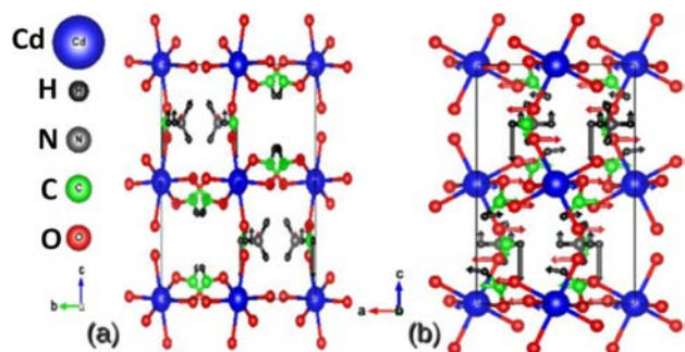
Figure 3. Atomic displacement field superposed on the reference centric structure. (a) is a projection along [100] . (b) shows a projection along [010] . Lengths of vectors are proportional to the corresponding atomic displacement.
