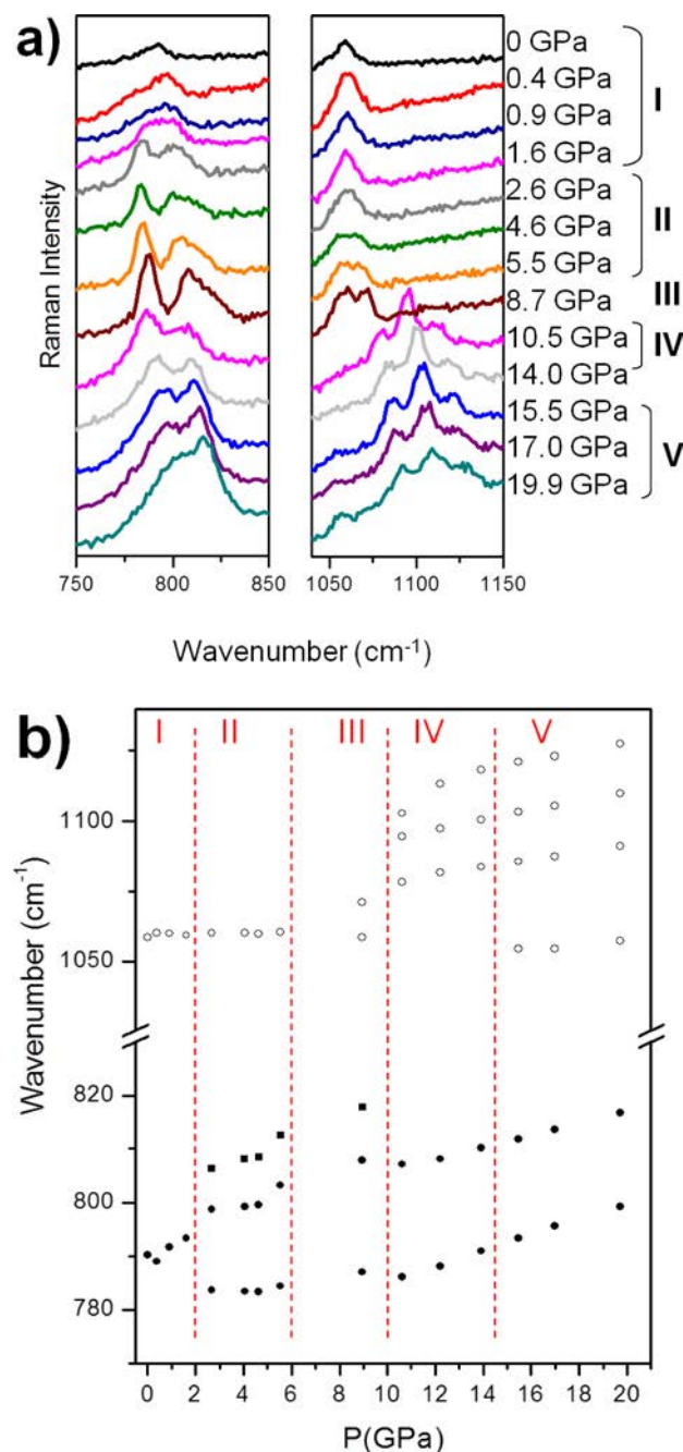
Figure 5. (a) Detail of the Raman spectra corresponding to the spectral ranges of 750–850 and 1040–1150 \text{cm}^{-1} . (b) Wavenumber vs pressure plots of the Raman modes corresponding to \nu_3 ( \text{HCOO}_3^- ) (symmetric O-C-O bending) and \nu_6 ( \text{HCOO}_3^- ) (out of plane H-C mode), represented as closed and open circles, respectively. The vertical lines signal approximate pressures at which the phase transitions take place.
